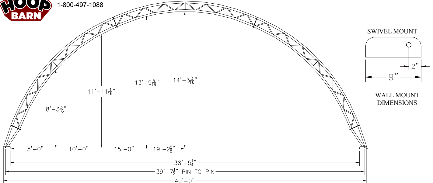
INTERIOR CLEARANCE
