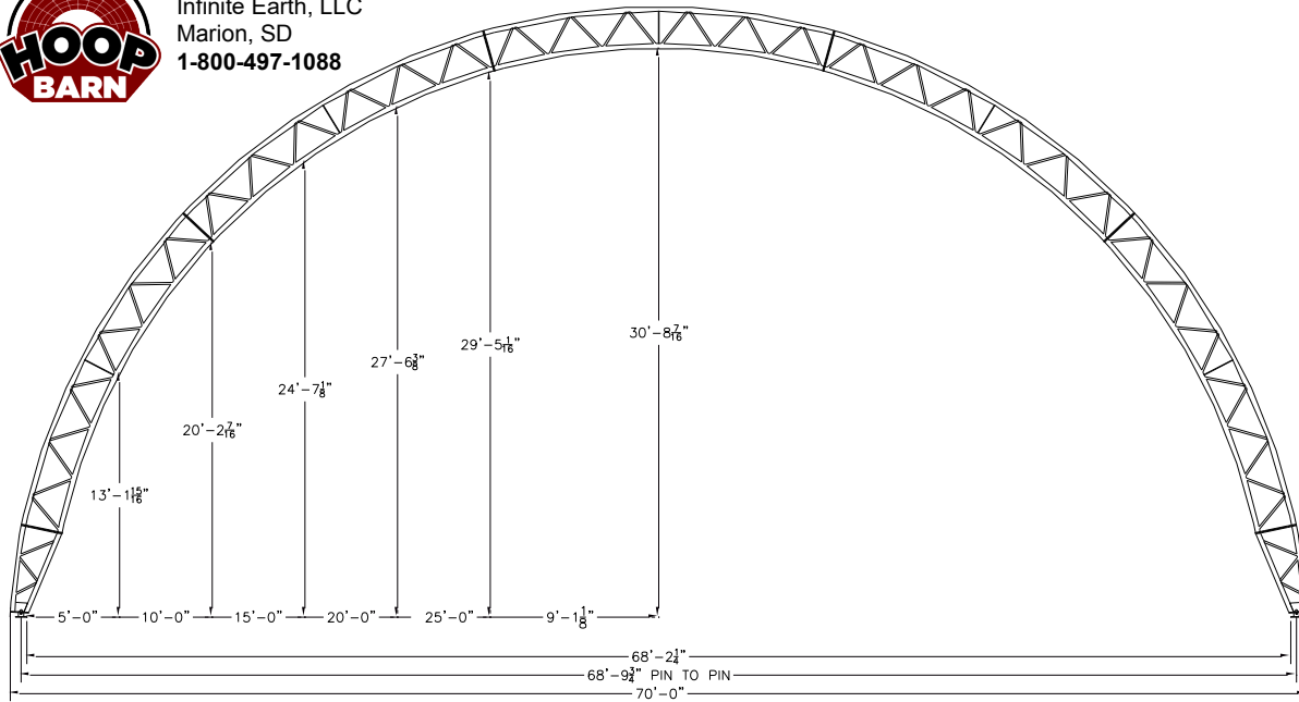
INTERIOR CLEARANCE
