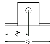
WALL MOUNT DIMENSIONS
